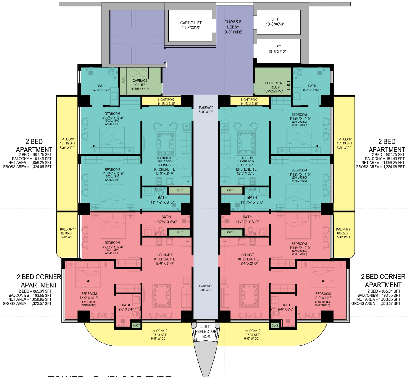
TOWER - B (FLOOR TYPE - 1) TOTAL FLOOR AREA FROM F.A.R = 5,232.29 SFT
